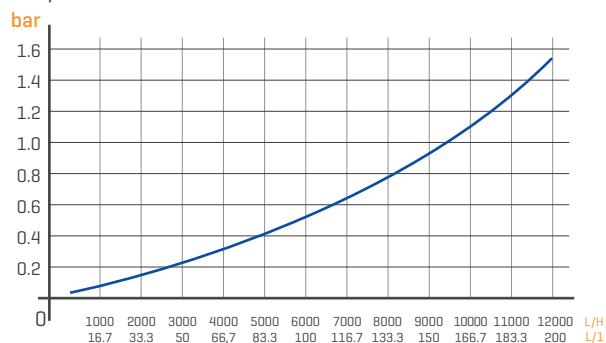
PRESSURE LOSS DIAGRAM 1"1/4 VERSION
